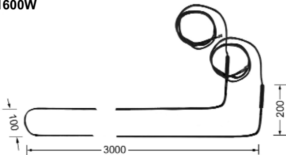
ME1186-1 1600W
