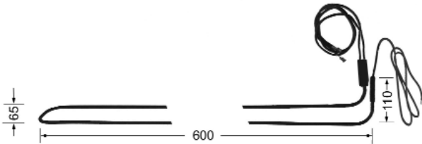
ME1206-2 600W
