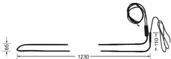
ME1205-9 1600W
