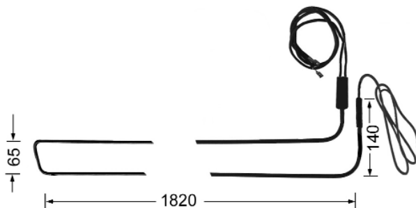
ME1206-4 1200W
