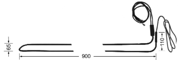
ME1205-2 600W
