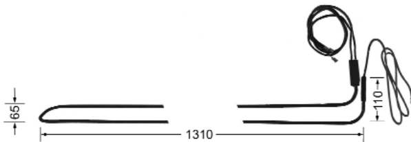
ME1205-7 800W
