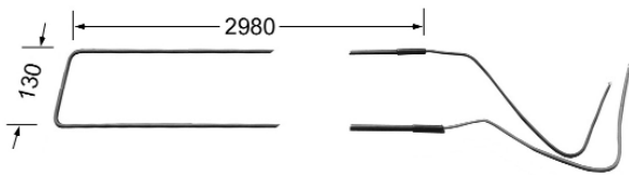
ME1186-1 1600W
