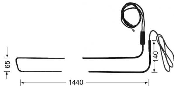
ME1206-3 900W
