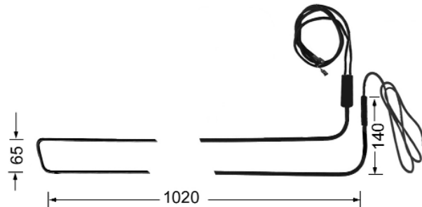
ME1206-2 600W
